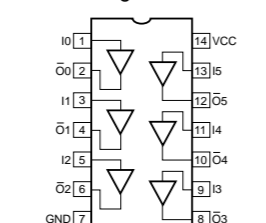
IC110: 74LCX14MTCX Low Voltage Hex Inverter
