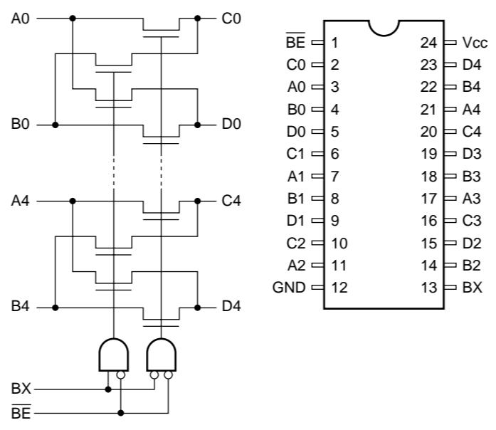
IC224-227: FST3383MTC 10-Bit Low Power Bus-Exchange Switch
