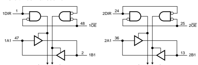
IC113-120: SN74LVCHR16245AGR 16-bit Bus Transceiver
