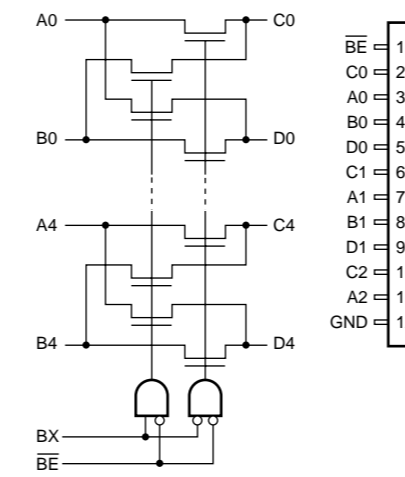
IC302-303, 307-310: FST3383MTC 10-Bit Low Power Bus-Exchange Switch
