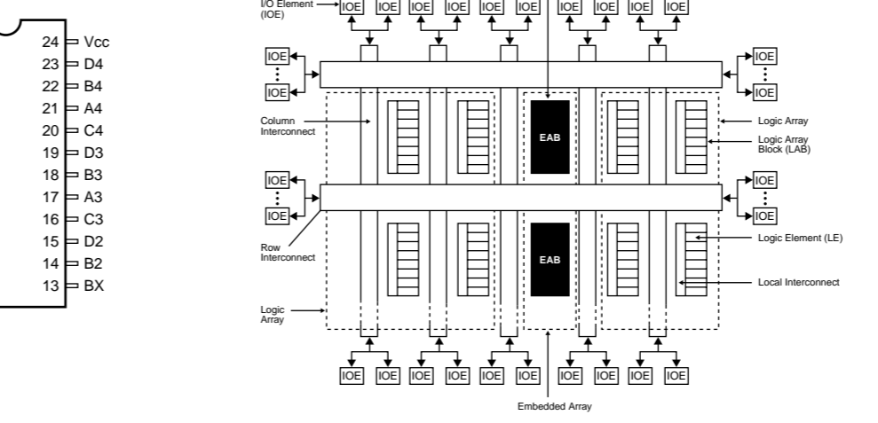
IC305: EP1K30TC144-3 FPGA
