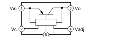
IC131: PQ070XZ5MZP Regulator
