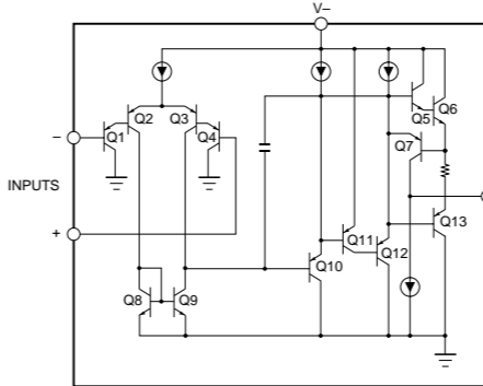
IC707: NJM2904V(TE1) Dual OP-Amp
