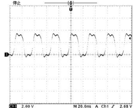
Point ① (Pin 6 of IC21)
