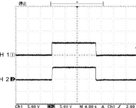
Point ③ CH 1 : Pin 1 of IC2 CH 2 : Pin 3 of IC2
