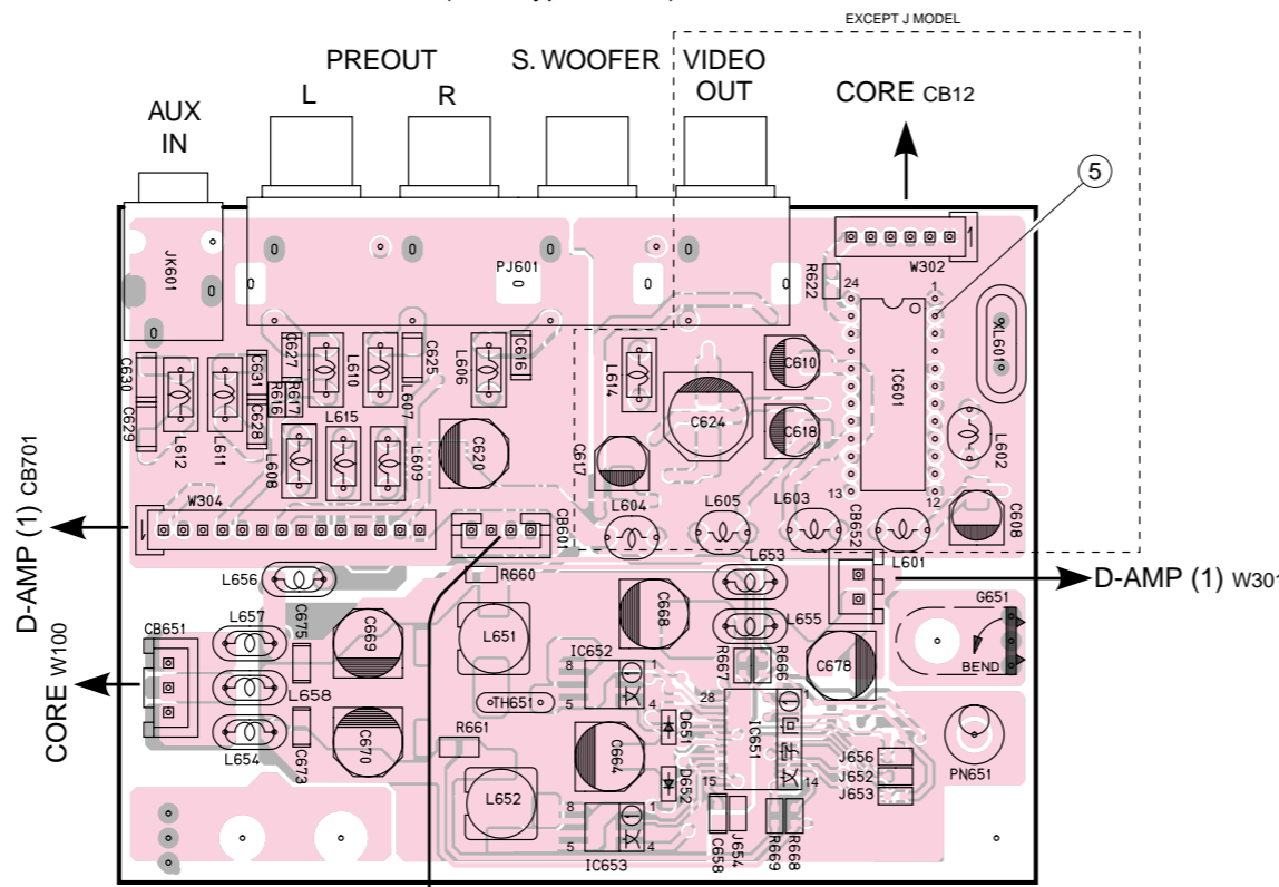
D-AMP (6) P. C. B. (Lead Type Device)
