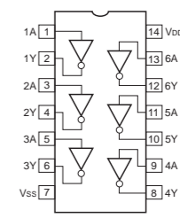
IC706 : TC74VHC04F Hex Inverters
