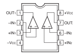
IC701 : NJM2904M-T1 Dual OP-Amp
