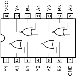
IC702 : HD74HC02FPEL Quad 2 Input NOR
