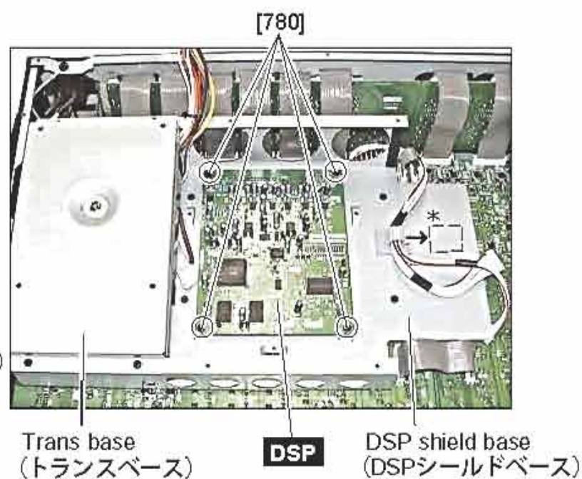
[780]: Bind Head Tapping Screw-S (+パインドSタイト) 3.0X6 MFZN2BL (EP630210)
