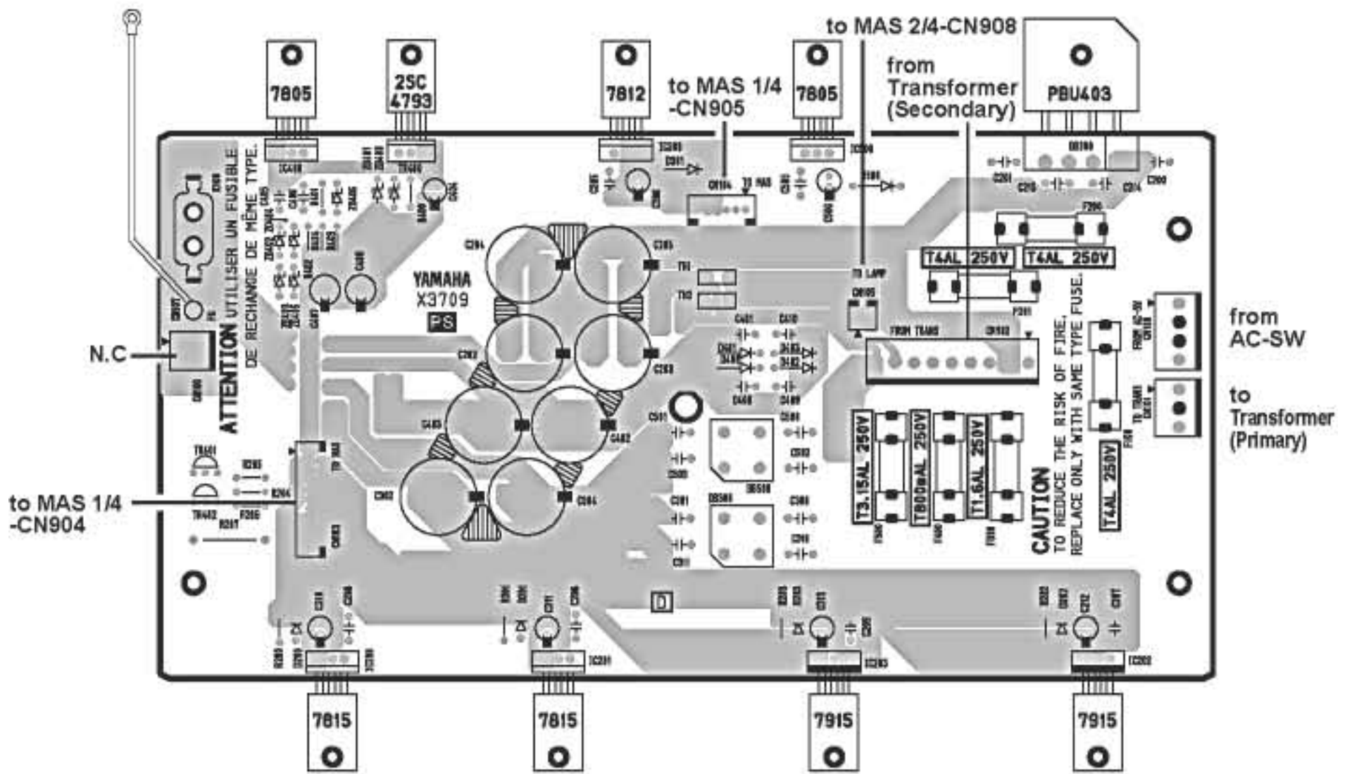
Component side (部品側)
