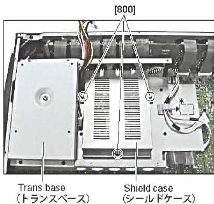
[800]: Bind Head Tapping Screw-S (+パインドSタイト) 3.0X6 MFZN2BL (EP630210)
