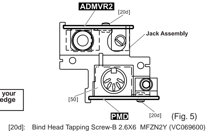
[20d]: Bind Head Tapping Screw-B 2.6X6 MFZN2Y (VC069600) (Fig. 5)
