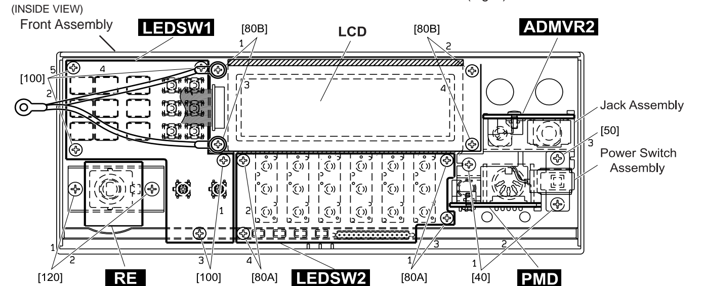
[40]: Bind Head Tapping Screw-B 3.0X6 MFZN2BL (EP600230) [100]: Bind Head Tapping Screw-B 2.6X6 MFZN2Y (VC069600) [50]: Bind Head Tapping Screw-B 2.6X10 MFZN2Y (VD791000) [120]: Bind Head Tapping Screw-B 3.0X6 MFZN2BL (EP600230) [80]: Bind Head Tapping Screw-B 2.6X10 MFZN2Y (VD791000) (Fig. 4)
