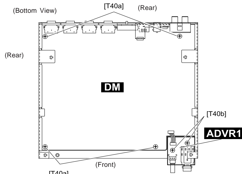
[T40a]: Bind Head Tapping Screw-B 3.0X6 MFZN2BL (EP600230) (Fig. 3)
