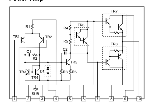
IC4 : STK404-050 Power Amp
