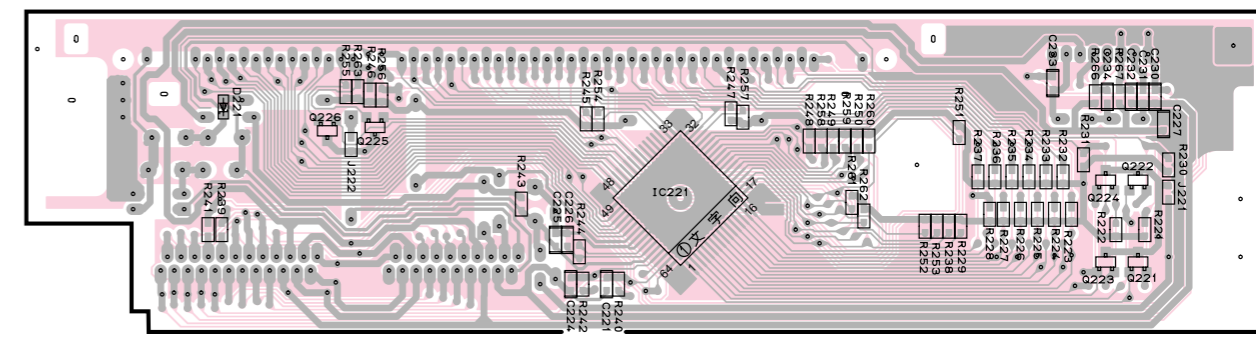
MAIN (3) P. C. B. (Surface Mount Device)
