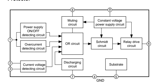
IC3 : TA7317P Protector
