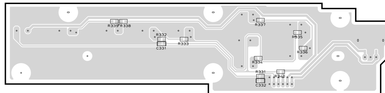
SUB (2) P.C.B. (Side B) Lead Free Solder Used
