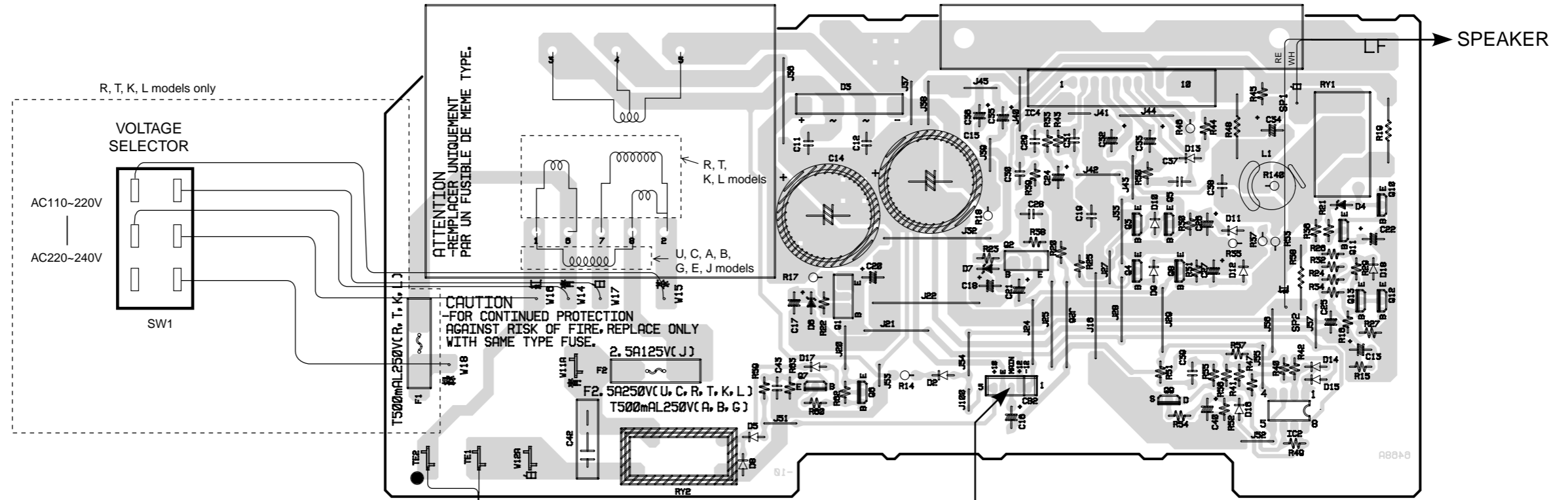
MAIN (1) P.C.B. (Side A)
