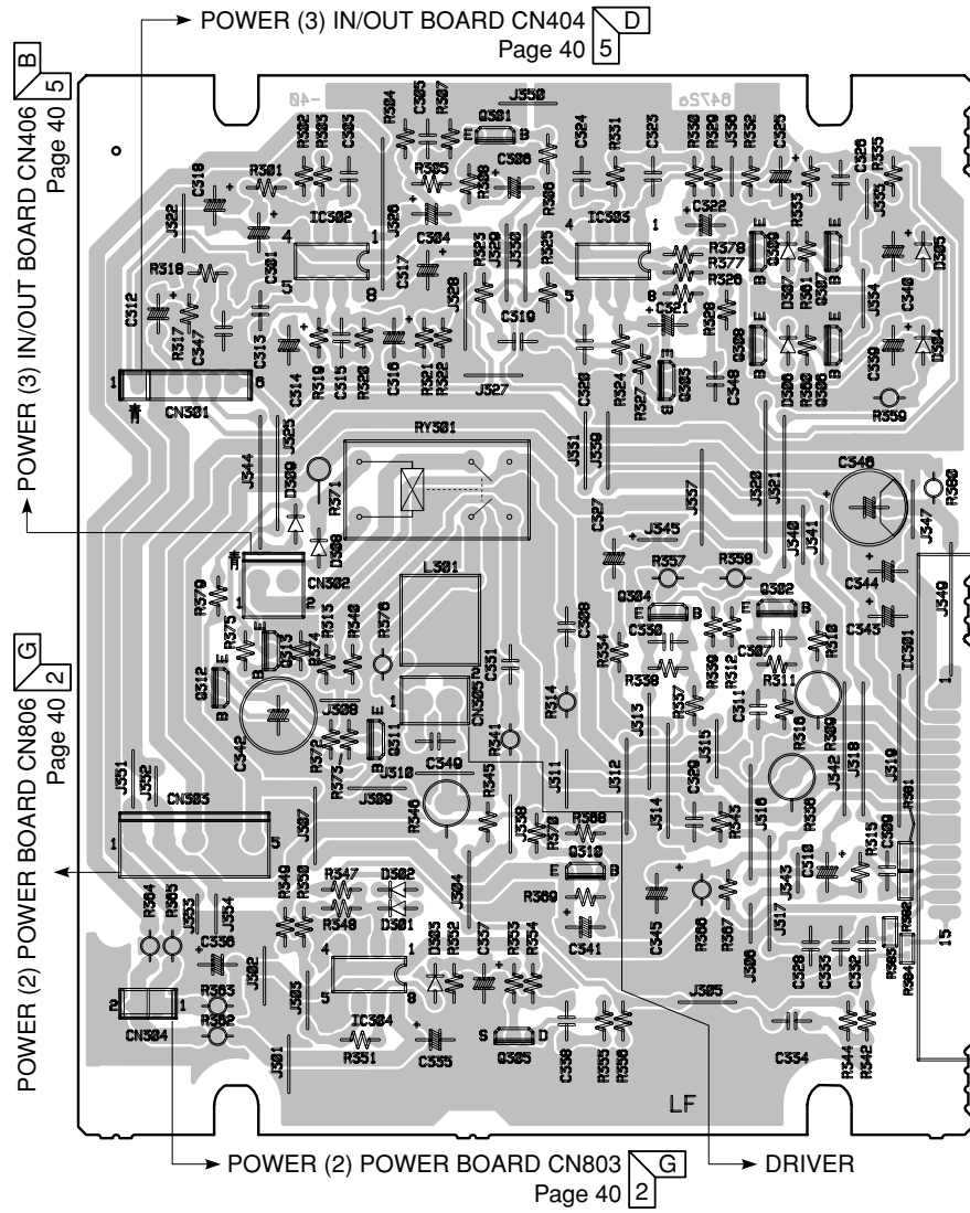
POWER (1) C/SW Board-Top View
