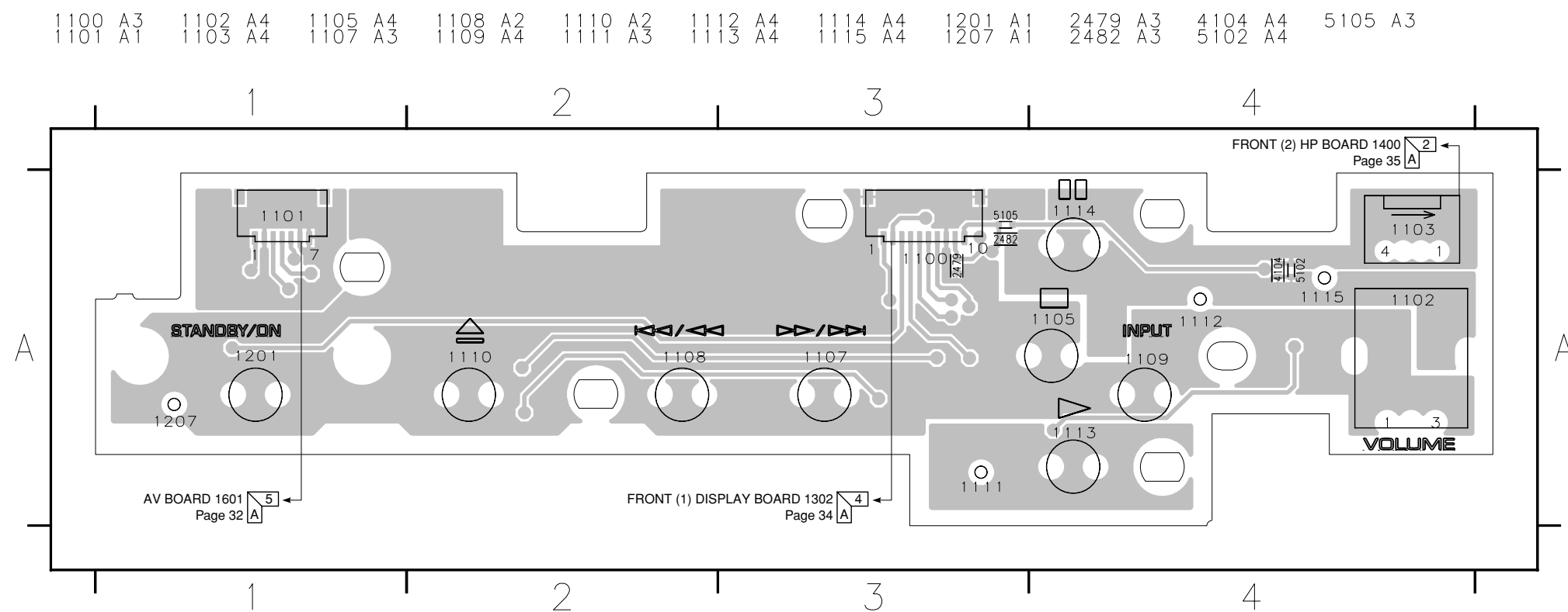
CONTROL Board-Top View
