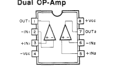
IC705, 706, 710 : μPC4570C Dual OP-Amp
