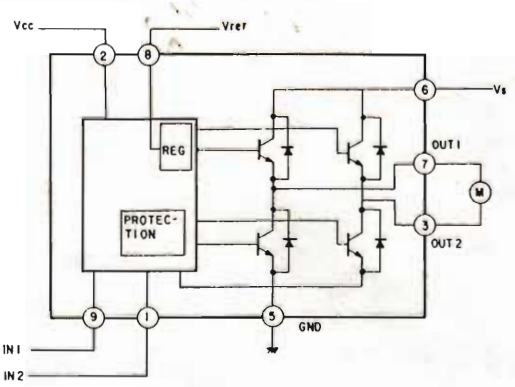
IC5 : TA7291S (Motor Driver)
