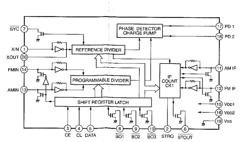
IC2 : LM7000N PLL Controller
