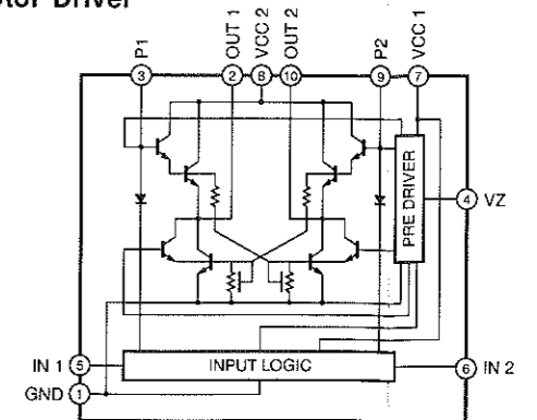
IC505 : LB1641 Motor Driver
