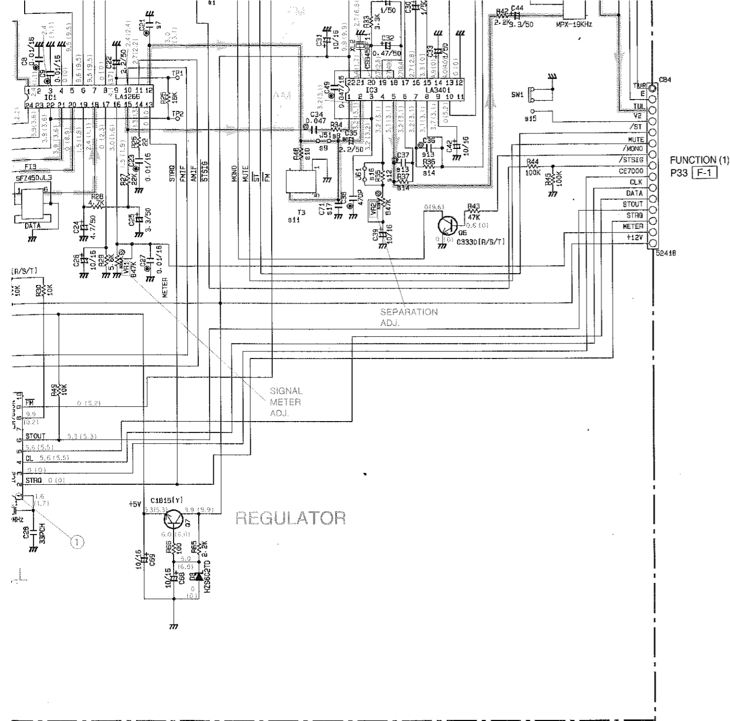
IC2 : LM7000N PLL Controller
