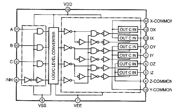
IC503, 504 : \mu PD4053BC Triple 2-Channel Multiplexer/Demultiplexer
