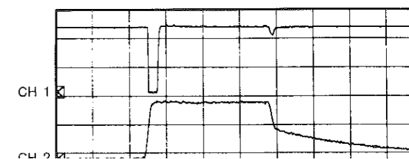
Point ③ (CH 1: Pin 10 of IC301) (CH 2: Emitter of Q303) V: 2V/div ..... CH1 V: 2V/div ..... CH2 H: 0.5sec/div DC range 1:1 probe (This waveform is not available by pushing the power switch ON and OFF.)
