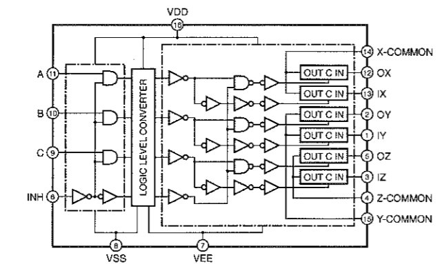
IC503, 504 : \mu PD4053BC Triple 2-Channel Multiplexer/Demultiplexer
