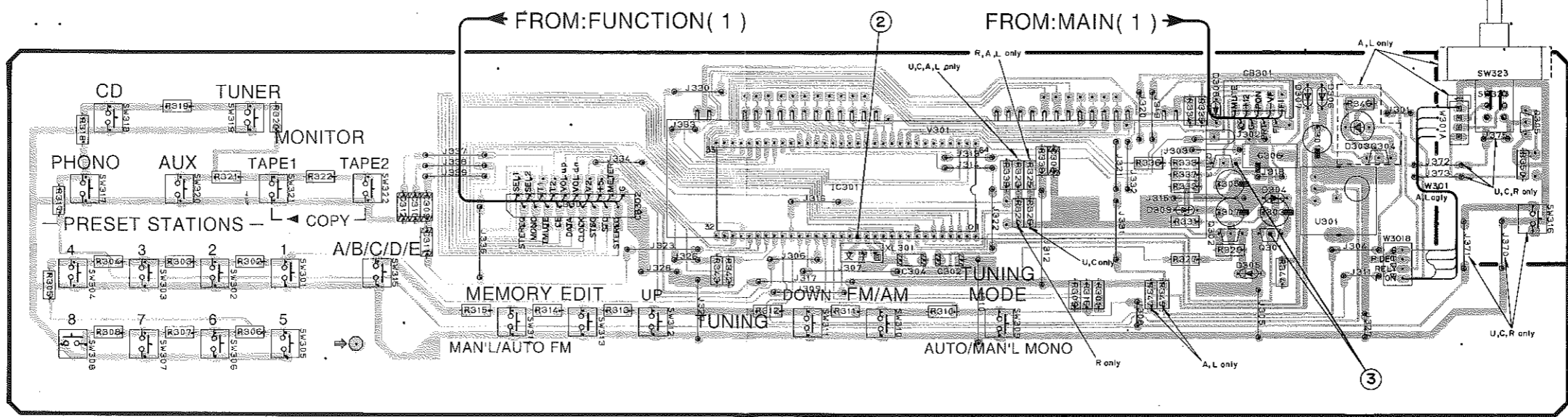
P.C.B. OPERATION (1)
