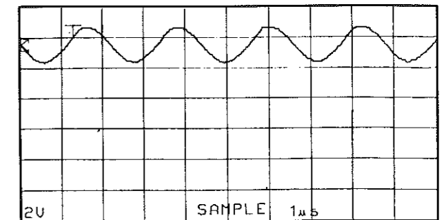
Point ⑤ (Pin 21 of IC3) V: 2V/div H: 1μsec/div DC range 1:1 probe
