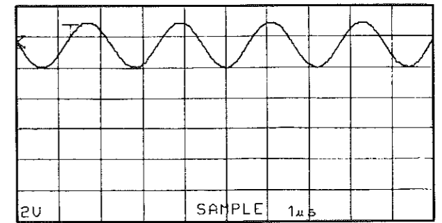
Point ⑥ (Pin 1 of IC4) V: 2V/div H: 1μsec/div DC range 1:1 probe
