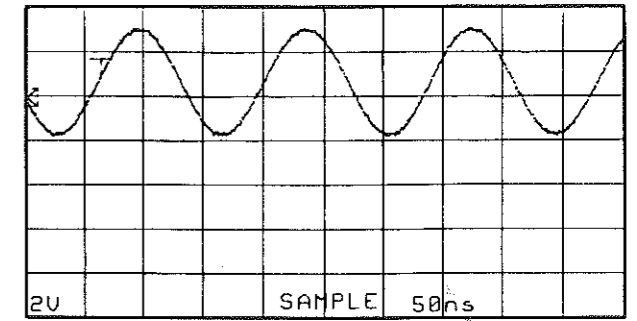
Point ④ (Pin 22 of IC2) V: 2V/div H: 50nsec/div DC range 1:1 probe
