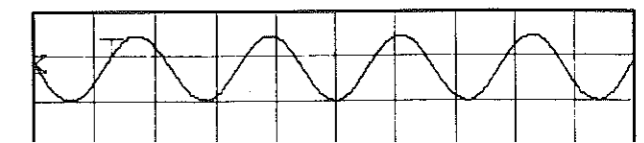
Point ⑥ (Pin 1 of IC4) V: 2V/div H: 1μsec/div DC range 1:1 probe
