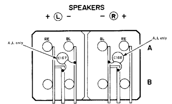
P.C.B. OPERATION (2)
