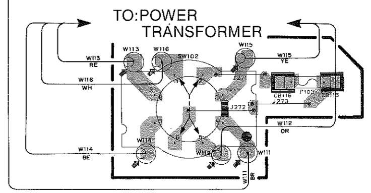
● R model P.C.B. MAIN ( 4 )
