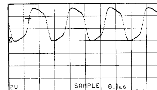
Point ② (Pin 15 of IC301) V: 2V/div H: 0.1μsec/div DC range 1:1 probe
