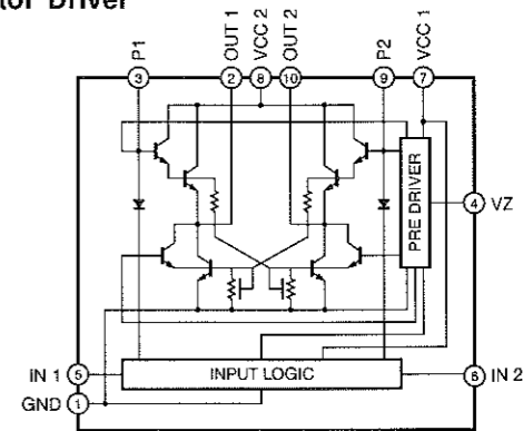
IC505 : LB1641 Motor Driver
