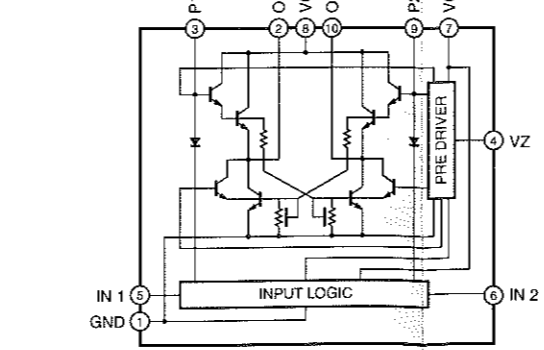
IC505 : LB1641 Motor Driver
