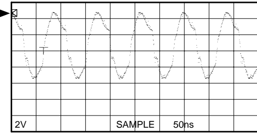
Point ⑥ Pin 28 of IC6 V : 2V/div H : 50nsec/div DC range 1 : 1 probe
