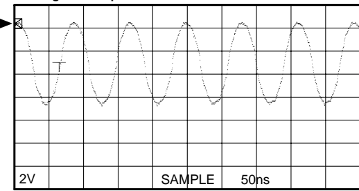
Point ⑤ Pin 13 of IC3 V : 2V/div H : 50nsec/div DC range 1 : 1 probe
