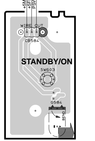
FUNCTION (5) P.C.B. (Lead Type Device)
