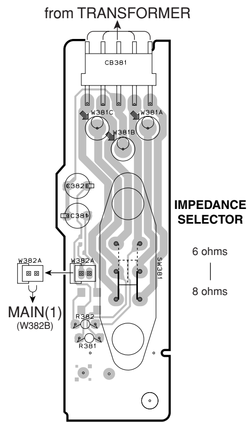
MAIN (4) P.C.B. (Side B)
