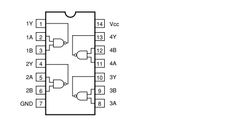
IC203: SN74AHC02PWR Quaduple 2-input positive-NOR gates
