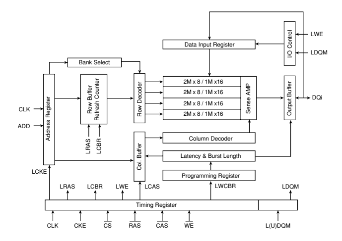
IC202: K4S641632K-UC60000 64 M synchronous DRAM
