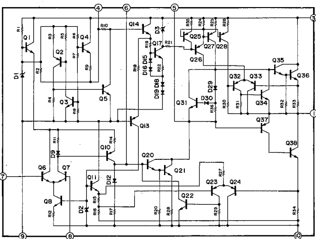
IC702 : μPC1188H Power Amp
