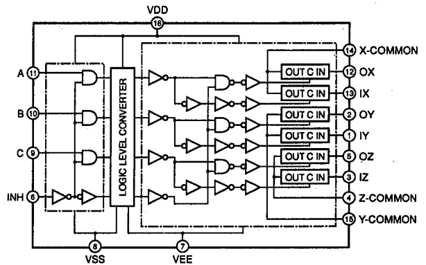
IC504 : TC4053BP Triple 2-Channel Multiplexer/Demultiplexer
