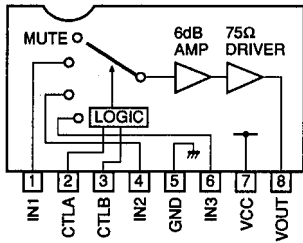
IC701 : BA7612N 3-Input Video Switch with 6dB Amp
