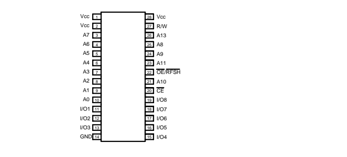
IC467 : LH5P832D-10 32768-word x 8 bit High Speed Pseudo Static RAM
