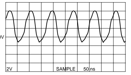
Point ① (Pin55 of IC466) V : 2V/div H : 50 nsec/div DC range 1 : 1 probe
