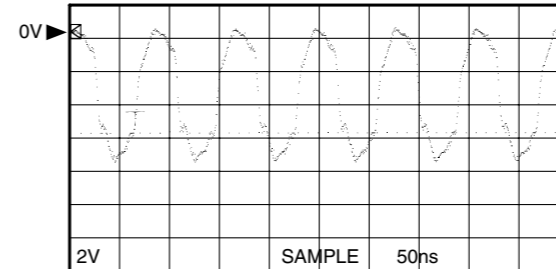
Point ⑥ Pin 28 of IC6 V : 2V/div H : 50nsec/div DC range 1 : 1 probe
