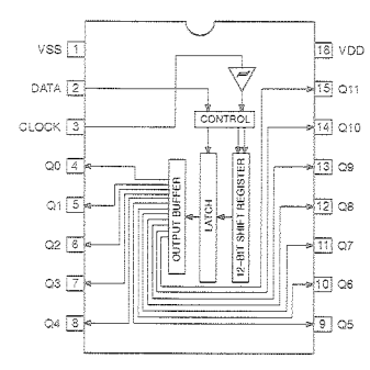
IC20 : BU2090 Serial In/Parallel Out Driver
