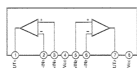
IC15, 17 : NJM4558L Dual OP-Amp
