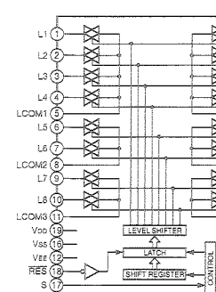
IC2 : LC78211 Analog Function Switch
