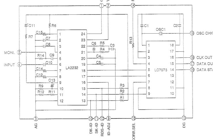
RDS Decoder & Controller
