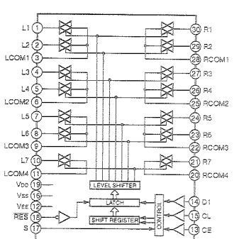
IC9 : LC78213 Analog Function Switch
