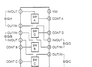
IC29 : μPD4068BC Quad Analog Switch/Multiplexer
