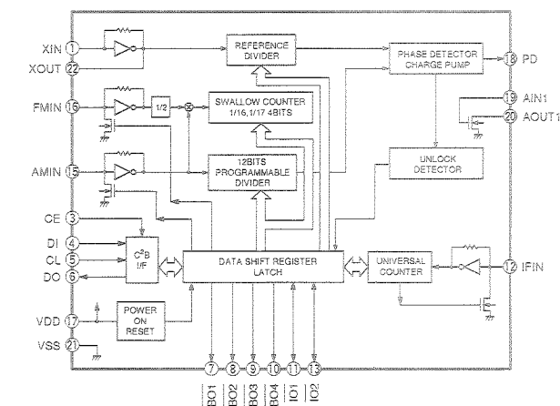
PLL Controller
