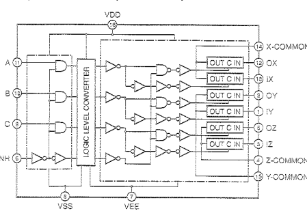
IC31 : TC4068BP Triple 2-Channel Multiplexer/Demultiplexer
