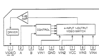
IC21, 24, 25 : LA7956 Video Switch
