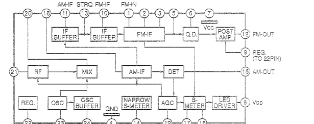
AM/FM IF
