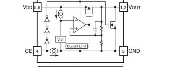
IC215: RP102K181D-TR Voltage regulator
