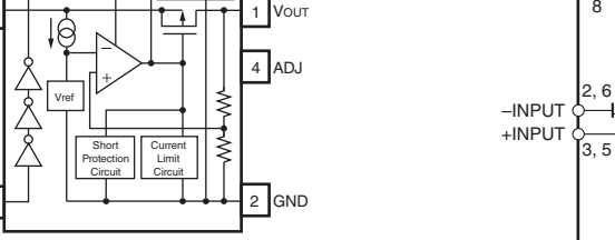
IC218: R1154H001C-T1-F Voltage regulator
