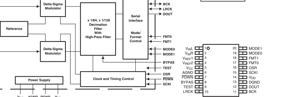
IC207: PCM1803DBR Stereo A/D converter
