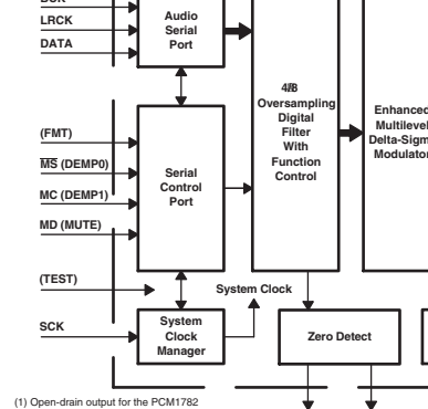
IC208: PCM1781BQR Audio digital-to-analog converter
