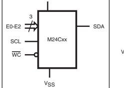
IC205: M24C02-RDW6TP 2 K-bit and 1 K-bit serial I2C bus EEPROM
