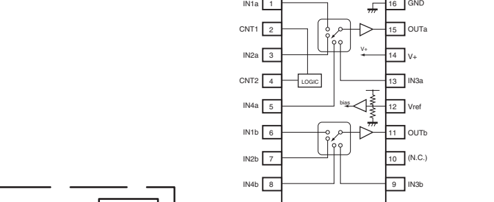
IC209: NJM2750M-TE2 4 input / 1 output stereo audio selector
