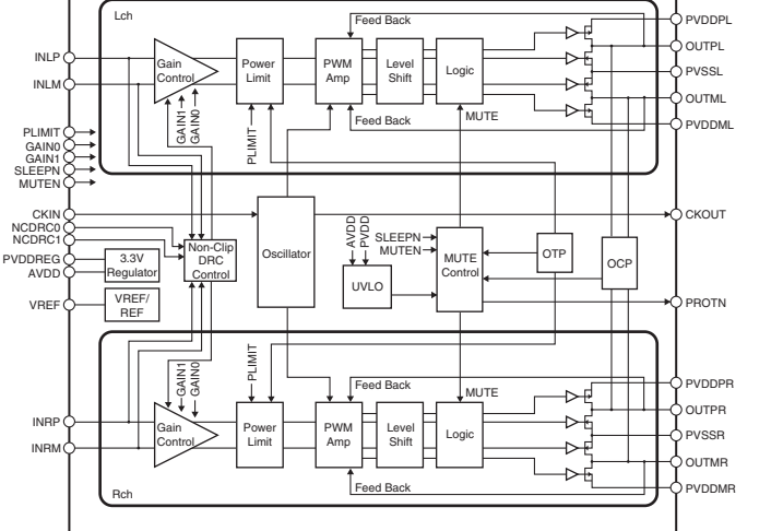
IC203: YDA147-SZE2 Digital audio power amplifier
