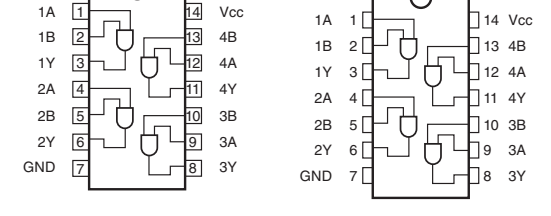
IC213: TC74VHC08AFT Quad 2-input AND gate
