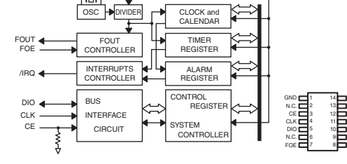
IC206: RX-4571SA A Real time clock module
