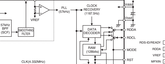
IC216: LC72725KM-UY-TLM-E RDS signal demodulation IC
