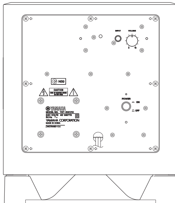
YST-SW010 (A model)
