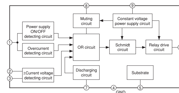
IC3 : TA7317P Protector
