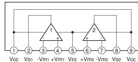
IC2, 4, 5: \mu PC4570HA Dual OP-Amp
