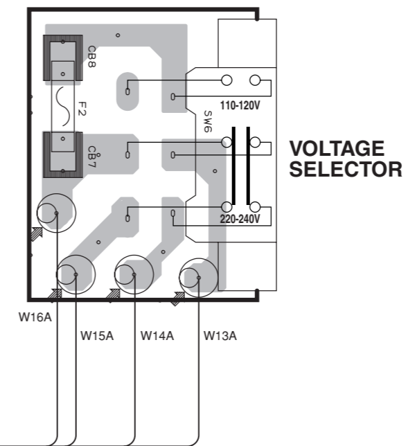
MAIN (9) P. C. B. (Lead Type Device)
